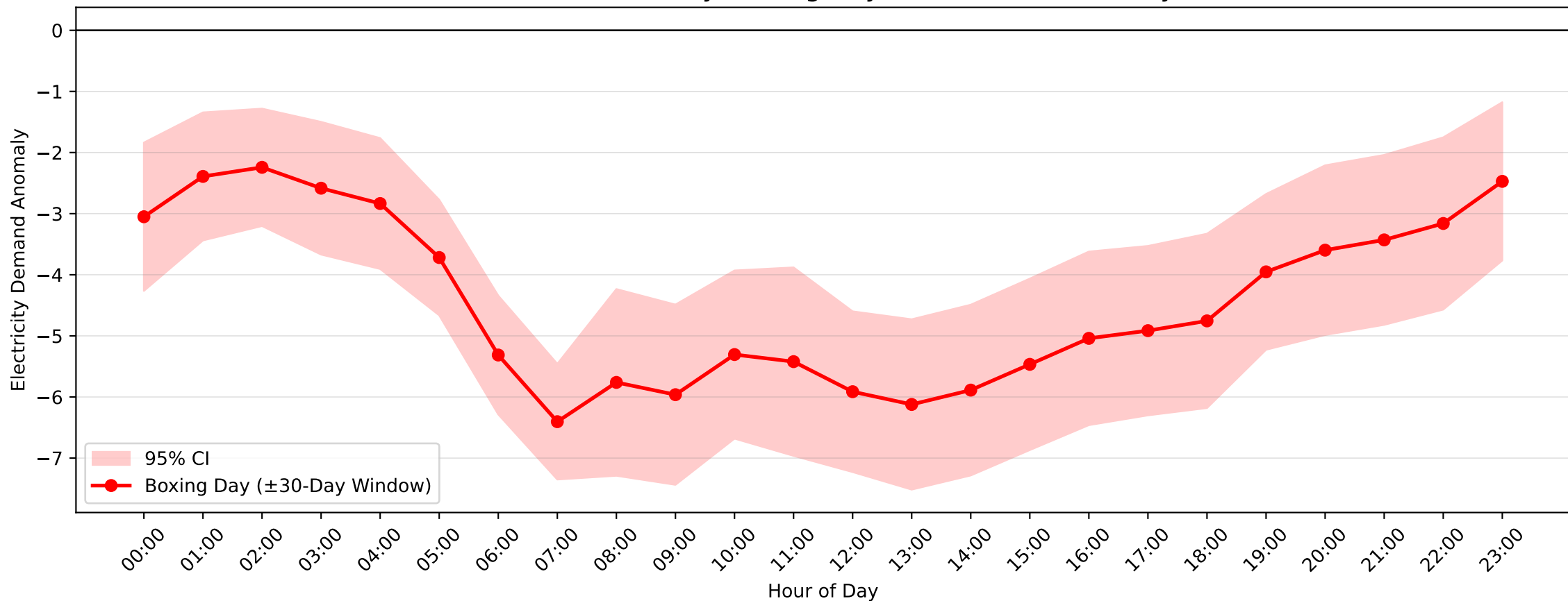
Matraverse Demand Anomaly: Boxing Day (2004-2017, \pm 30 -Day Window)
